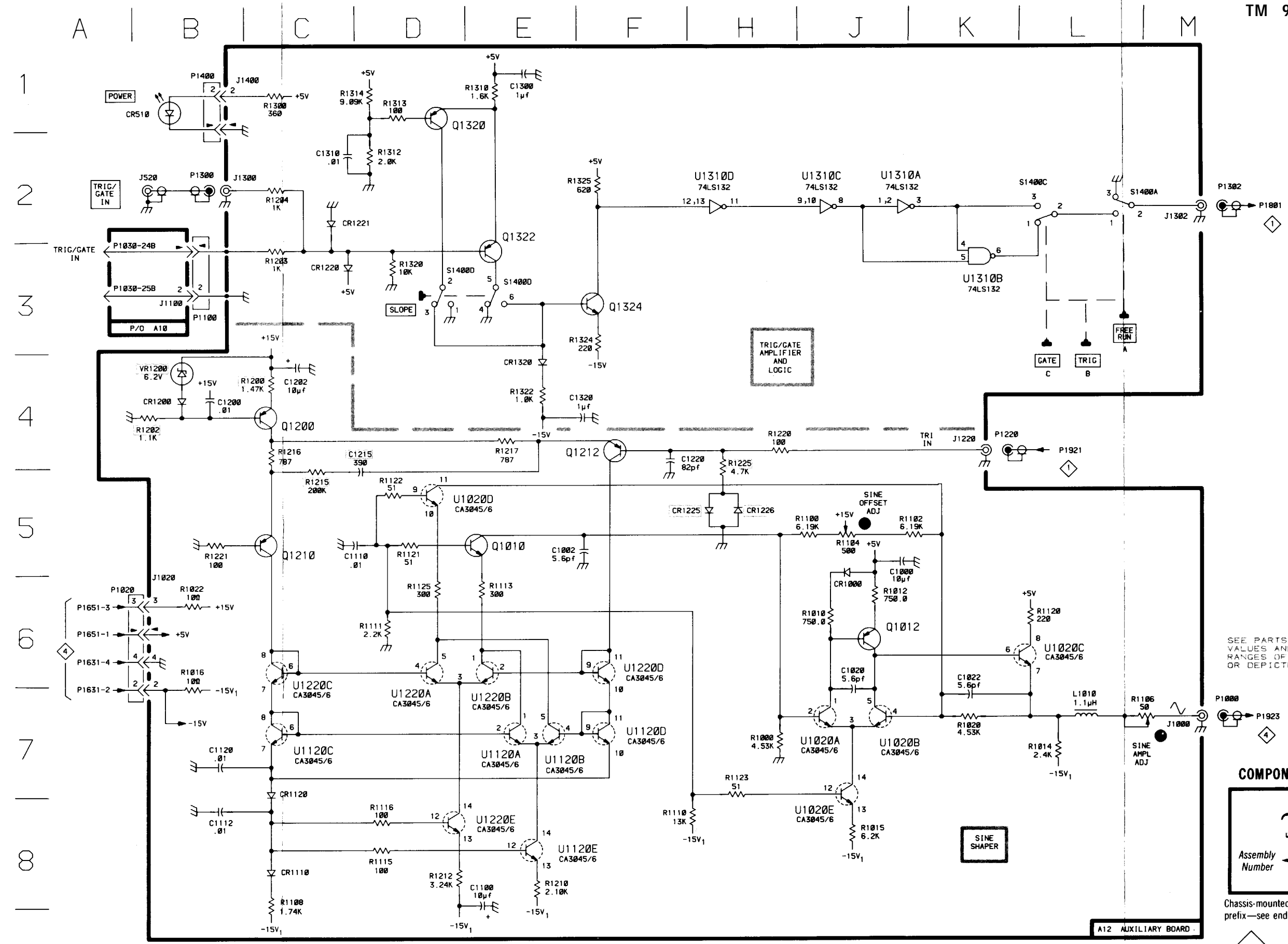
TRIG/GATE AND SINE SHAPER AMPLIFIER
